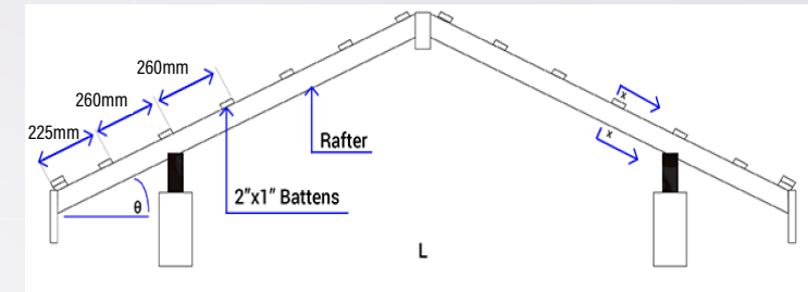
Minimum Roof Angle (θ) = 25°
