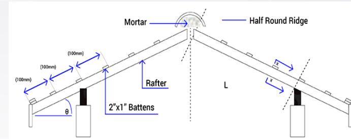
Minimum Roof Angle (θ) = 30°
